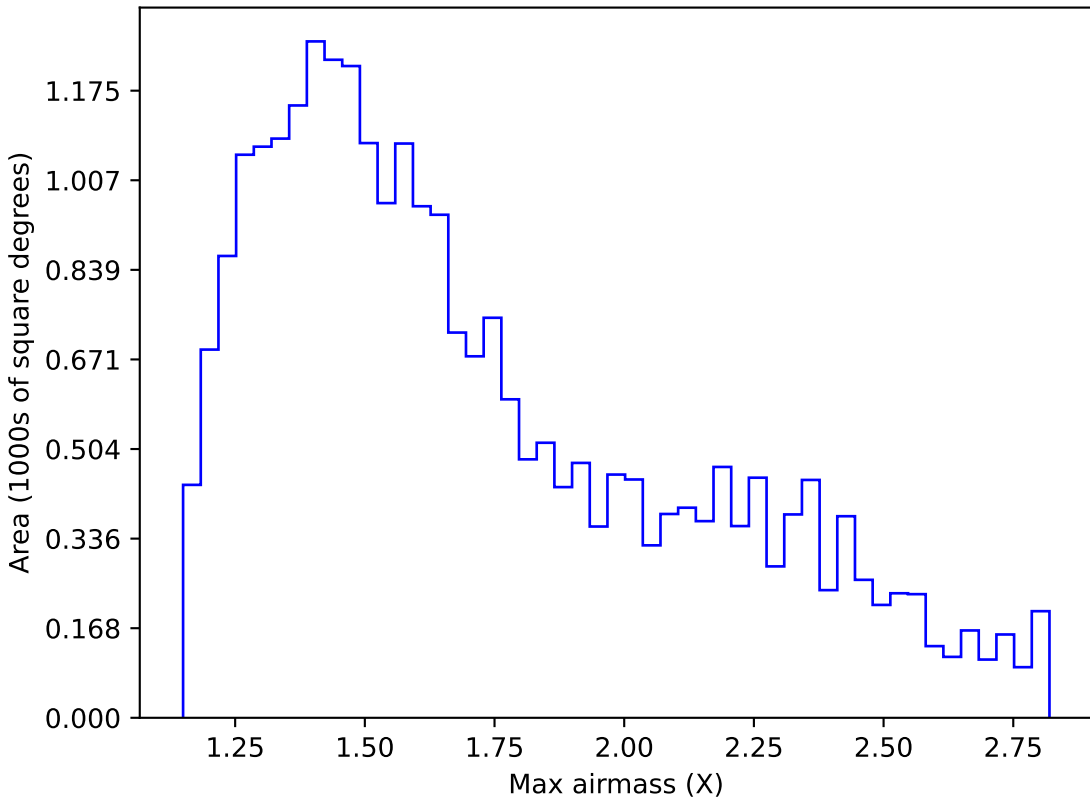
ddf_loaded_fl8_v3.4_10yrs Yr 1 i band: Max airmass
