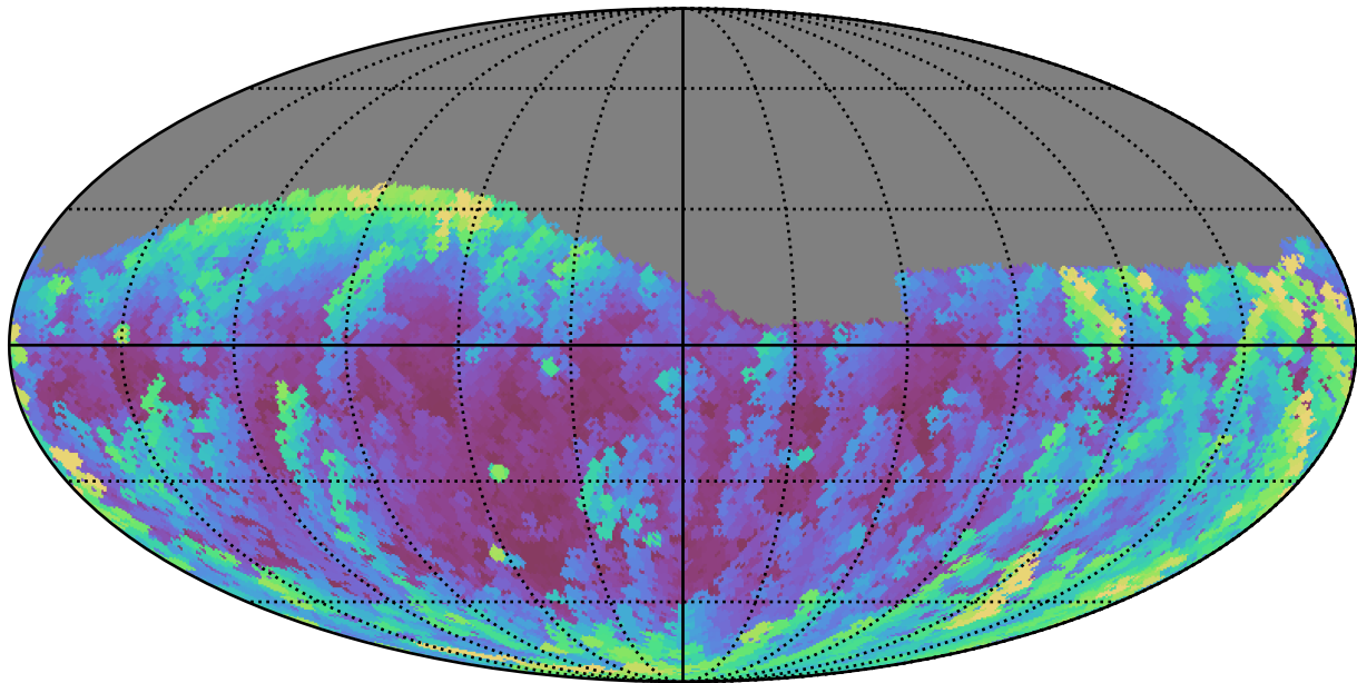
ddf_loaded_fl8_v3.4_10yrs Yr 1 g band: Max airmass
