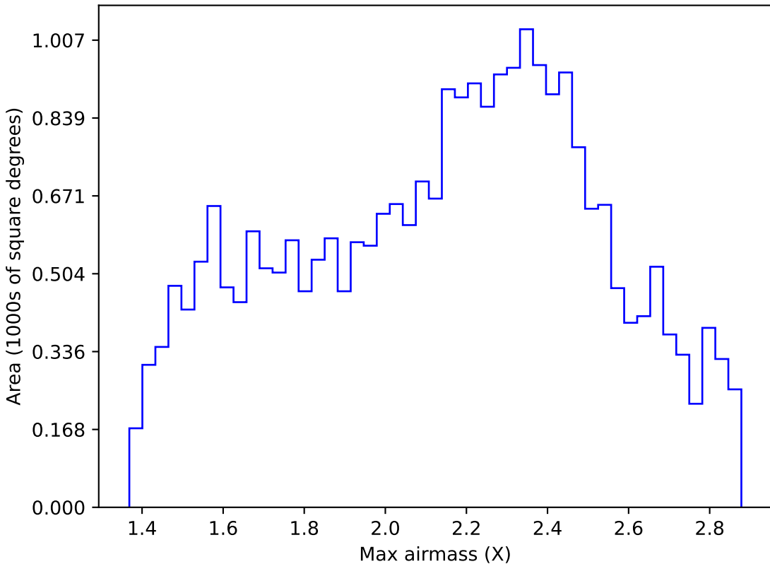
ddf_loaded_fl8_v3.4_10yrs Yr 1 all bands: Max airmass
