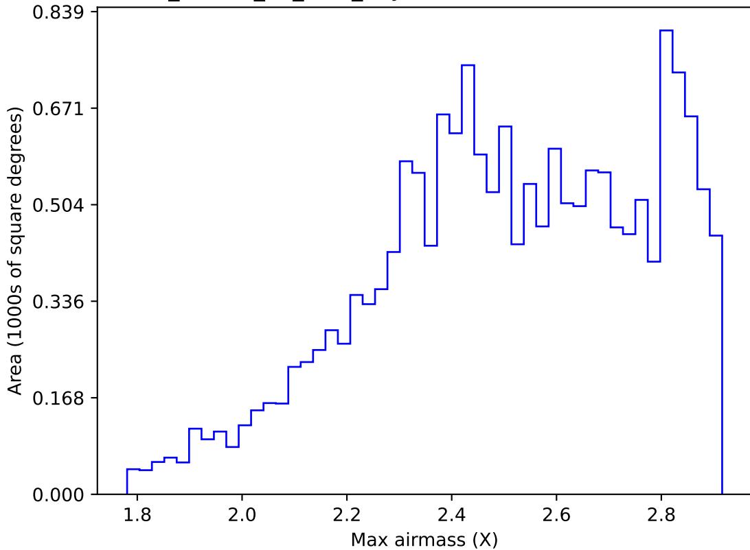
ddf_loaded_fl8_v3.4_10yrs WFD z band: Max airmass
