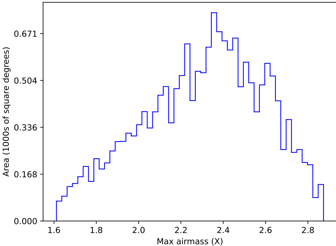
ddf_loaded_fl8_v3.4_10yrs WFD y band: Max airmass
