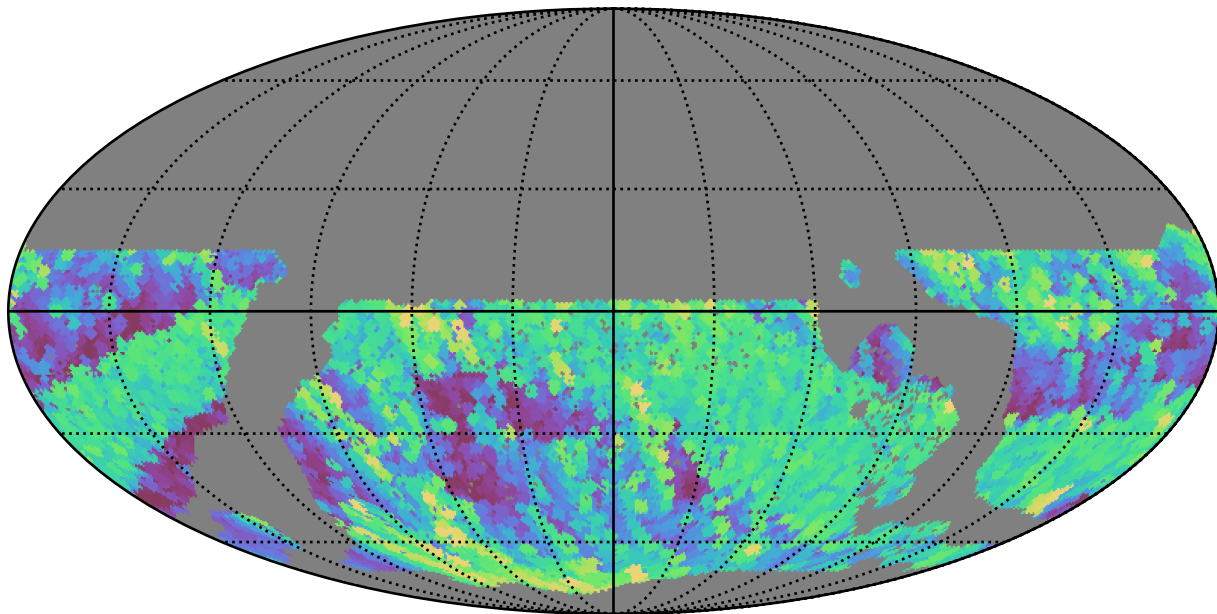
ddf_loaded_fl8_v3.4_10yrs WFD r band: Max airmass
