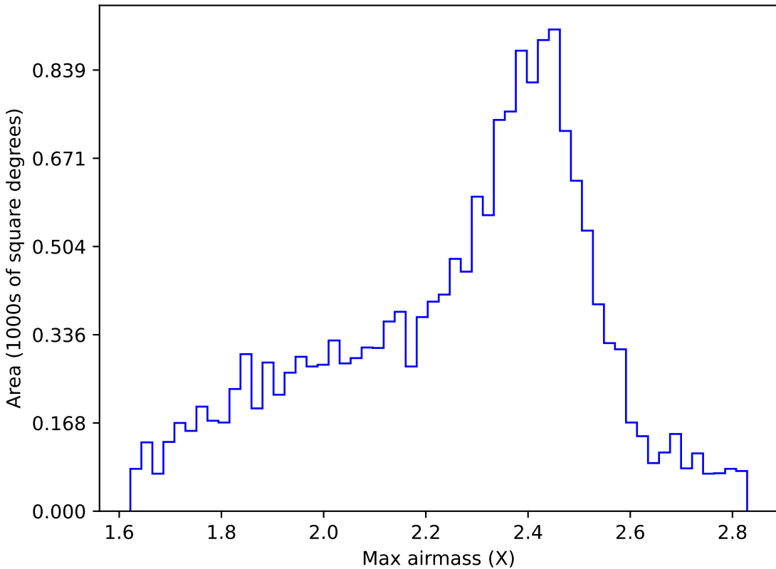
ddf_loaded_fl8_v3.4_10yrs WFD r band: Max airmass
