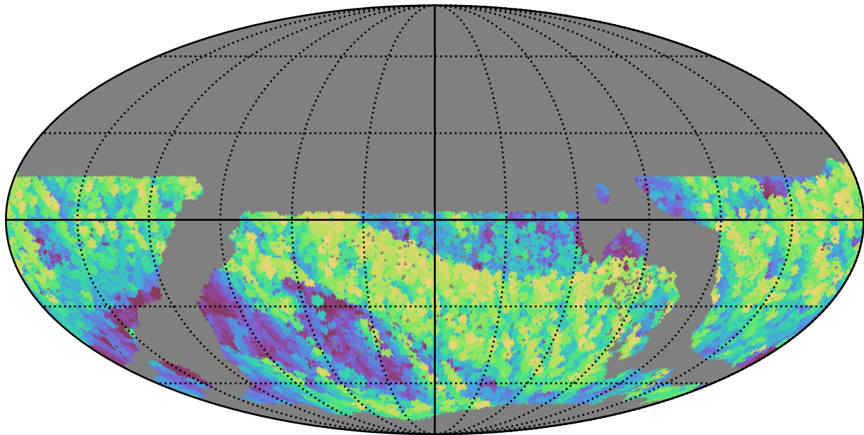
ddf_loaded_fl8_v3.4_10yrs WFD i band: Max airmass
