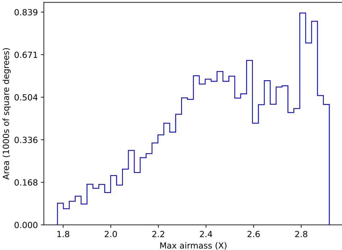
ddf_loaded_fl8_v3.4_10yrs WFD i band: Max airmass
