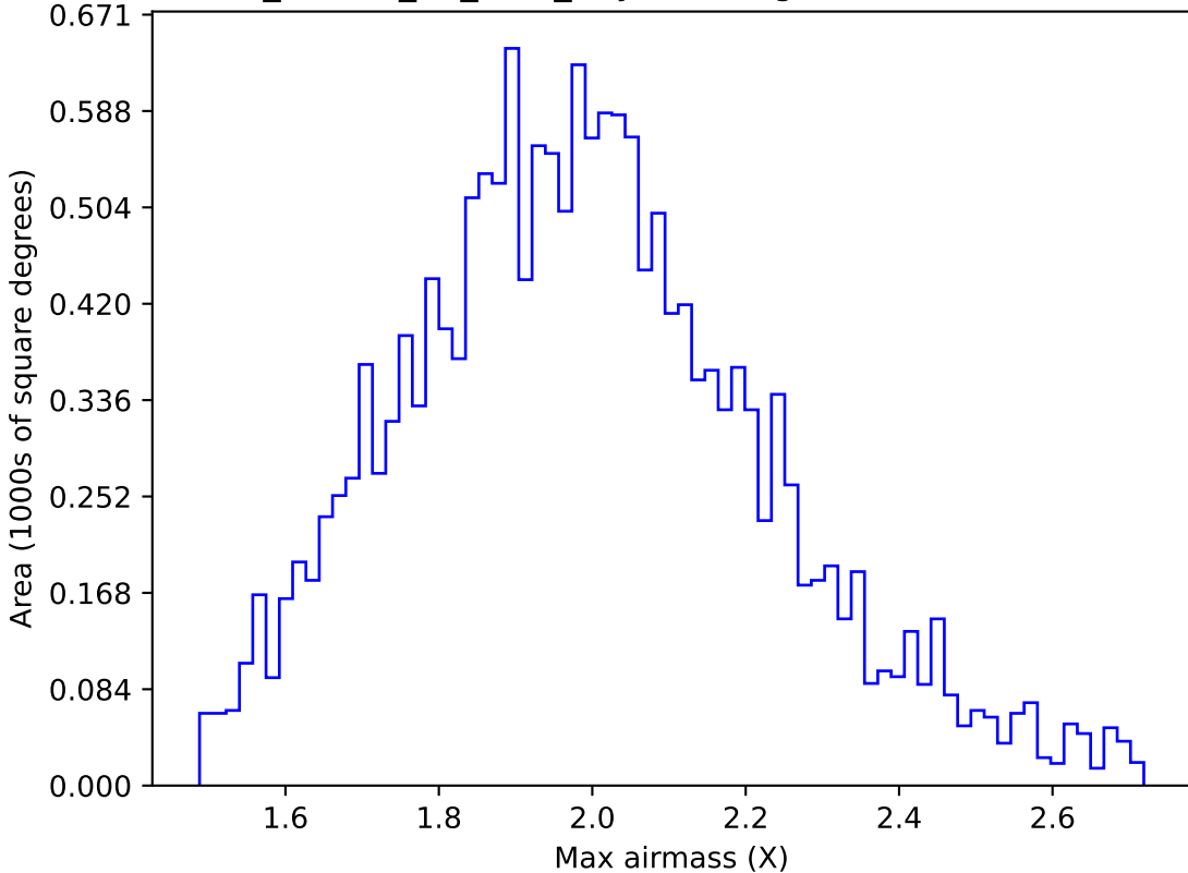
ddf_loaded_fl8_v3.4_10yrs WFD g band: Max airmass
