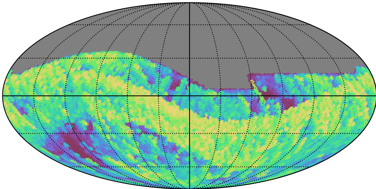
ddf_loaded_fl8_v3.4_10yrs All sky z band: Max airmass
