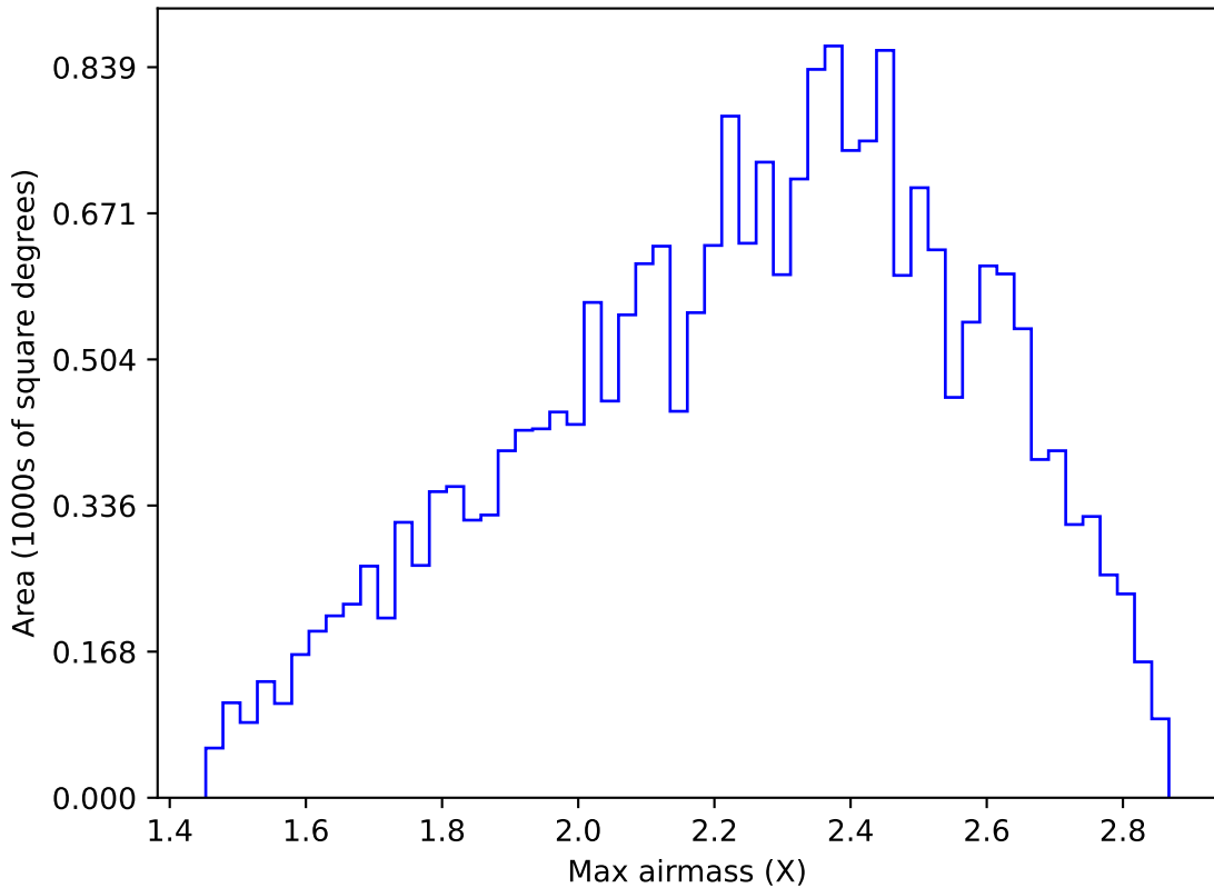
ddf_loaded_fl8_v3.4_10yrs All sky y band: Max airmass
