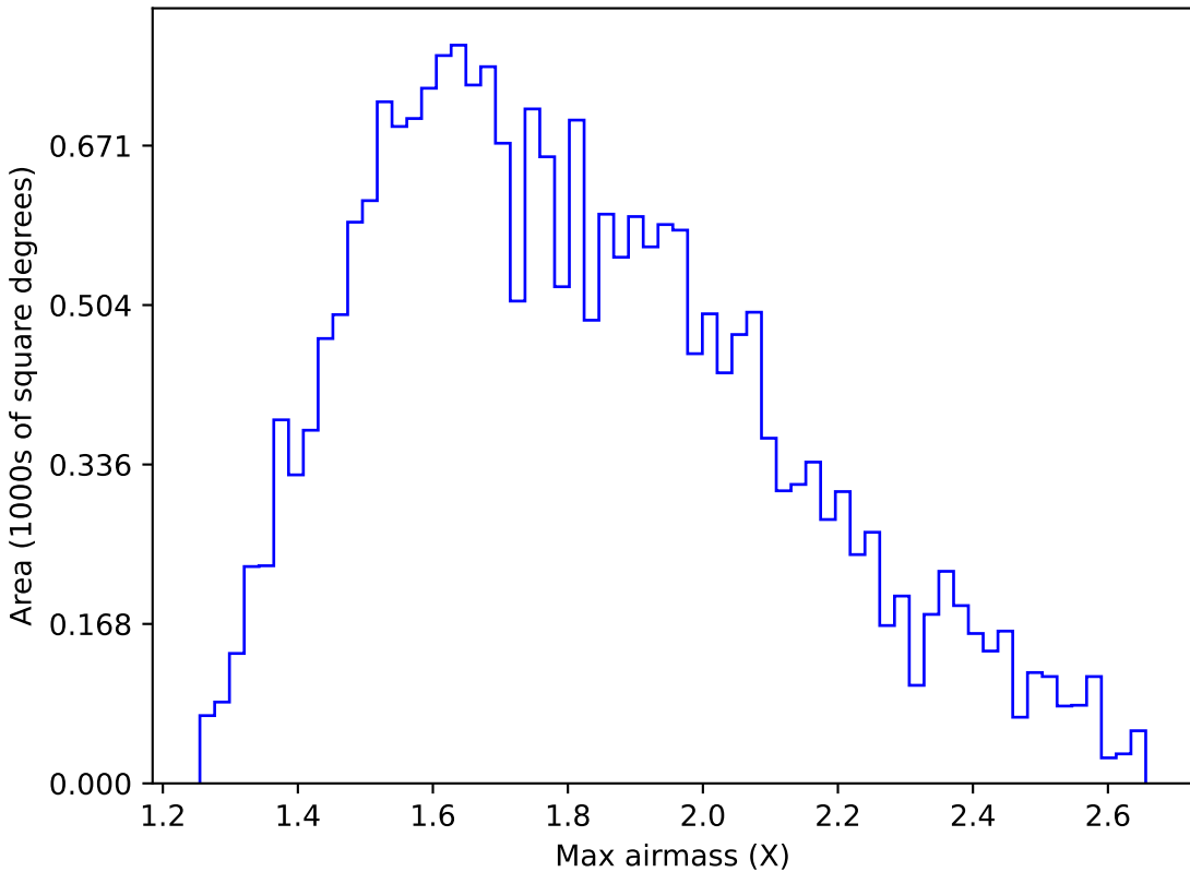
ddf_loaded_fl8_v3.4_10yrs All sky u band: Max airmass
