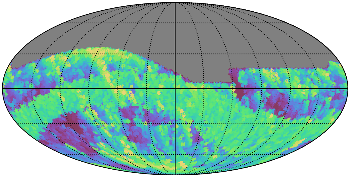
ddf_loaded_fl8_v3.4_10yrs All sky r band: Max airmass
