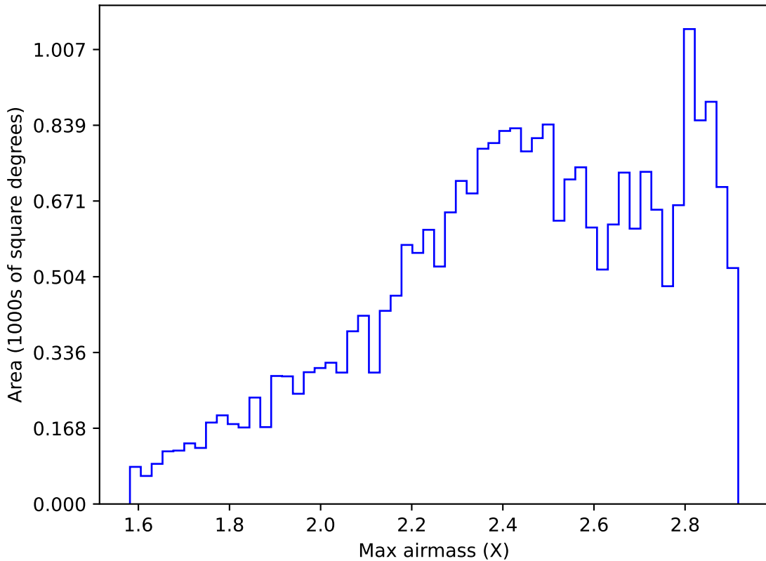
ddf_loaded_fl8_v3.4_10yrs All sky i band: Max airmass
