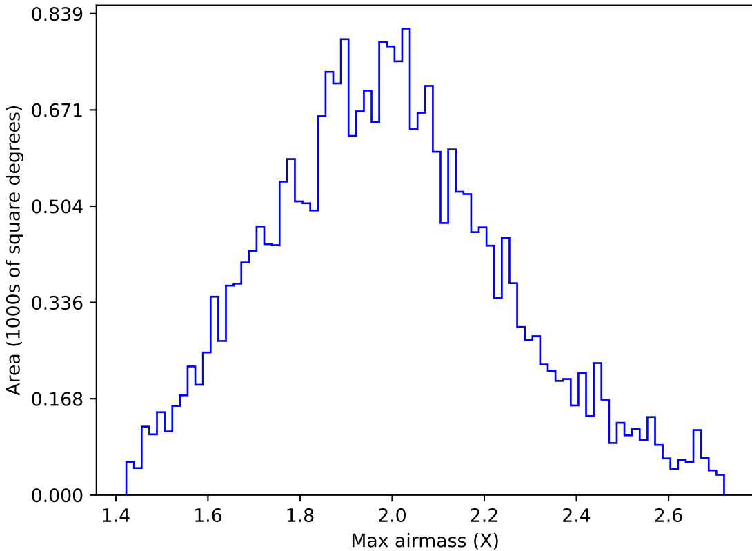
ddf_loaded_fl8_v3.4_10yrs All sky g band: Max airmass
