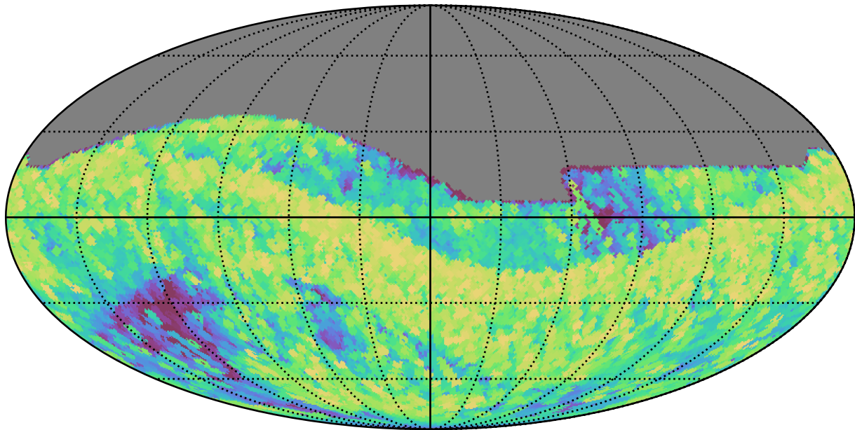
ddf_loaded_fl8_v3.4_10yrs All sky all bands: Max airmass
