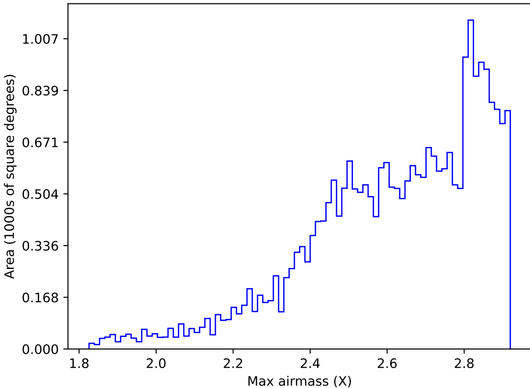
ddf_loaded_fl8_v3.4_10yrs All sky all bands: Max airmass
