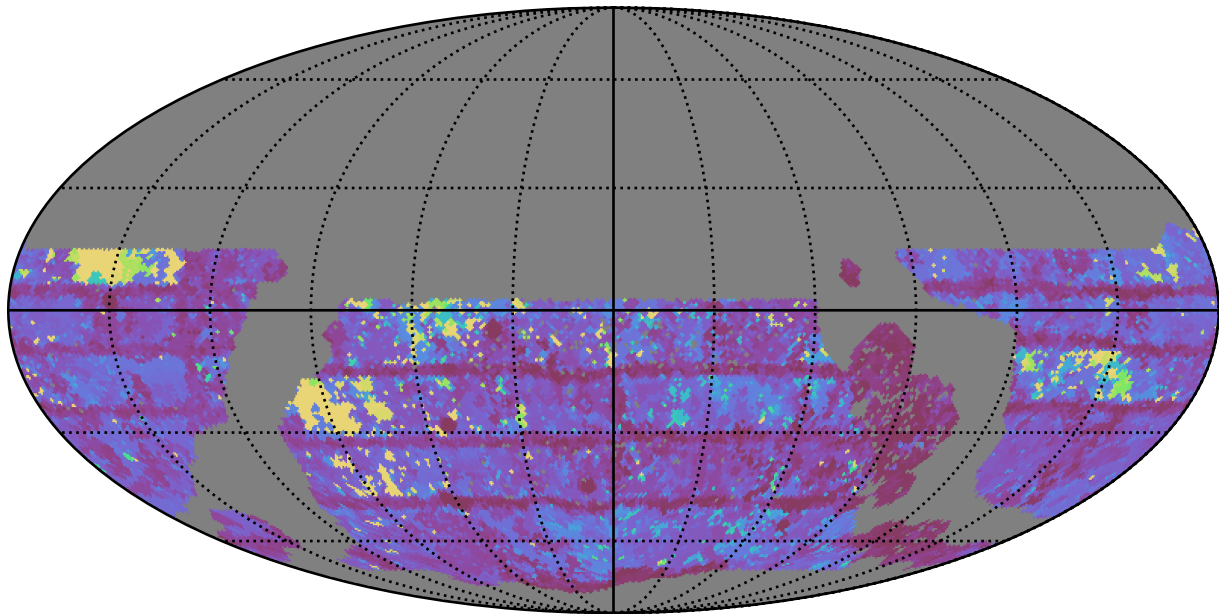
ddf_loaded_fl8_v3.4_10yrs WFD z band: Max Inter-Night Gap
