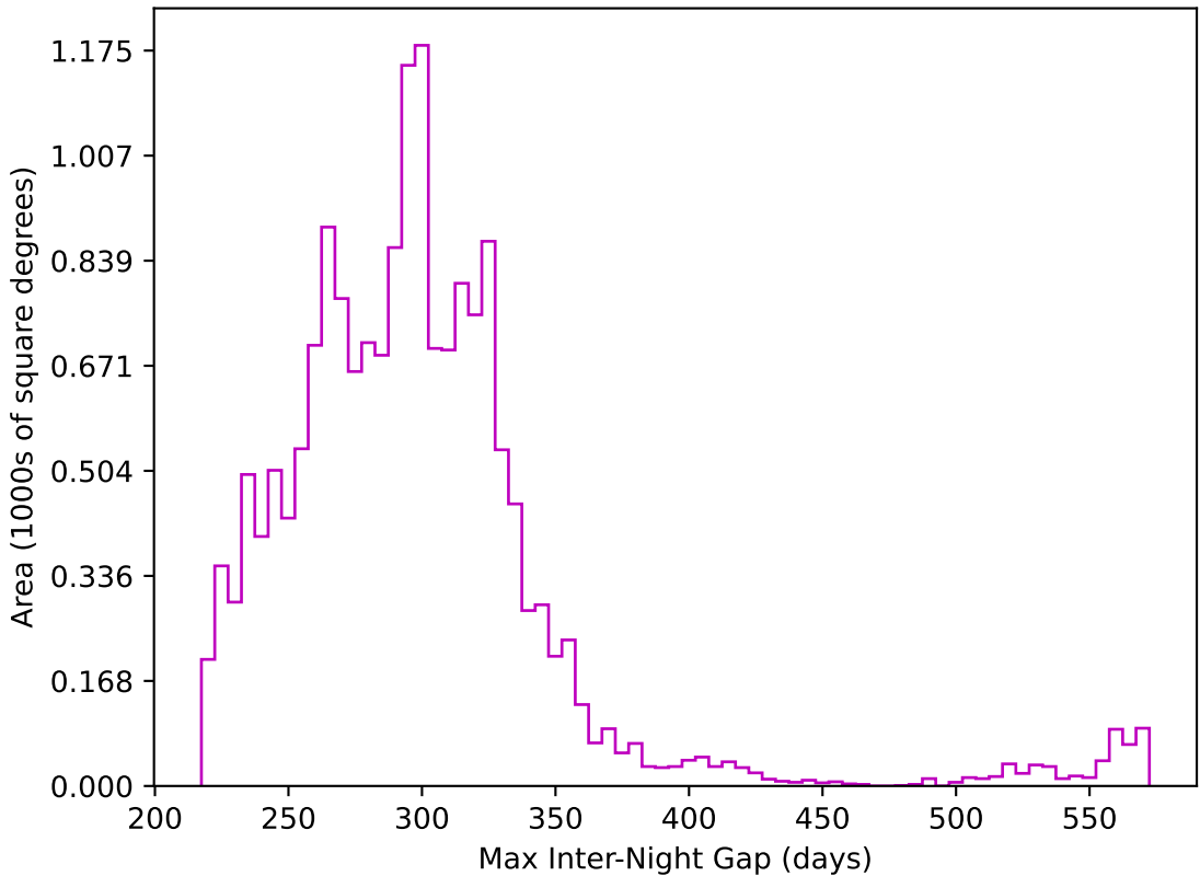
ddf_loaded_fl8_v3.4_10yrs WFD z band: Max Inter-Night Gap
