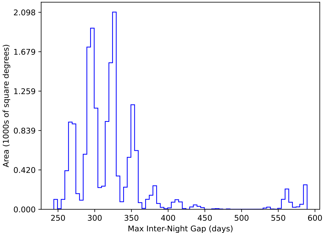
ddf_loaded_fl8_v3.4_10yrs WFD y band: Max Inter-Night Gap
