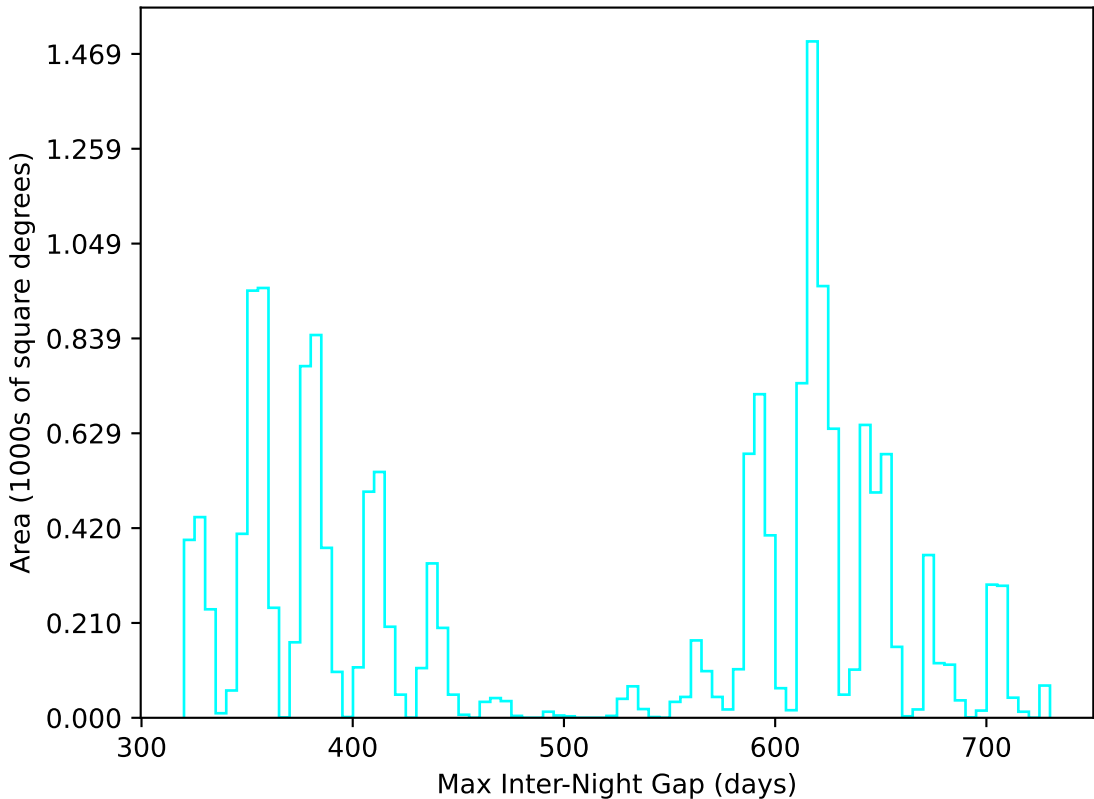
ddf_loaded_fl8_v3.4_10yrs WFD u band: Max Inter-Night Gap
