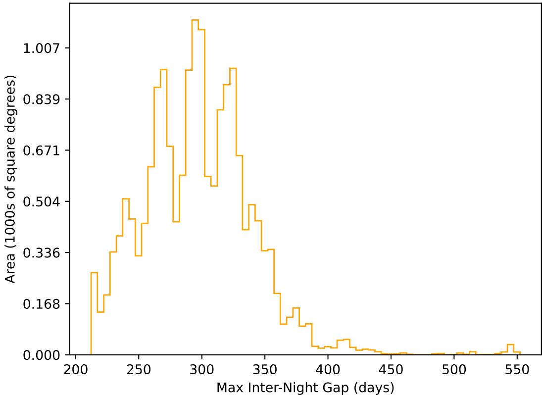
ddf_loaded_fl8_v3.4_10yrs WFD r band: Max Inter-Night Gap
