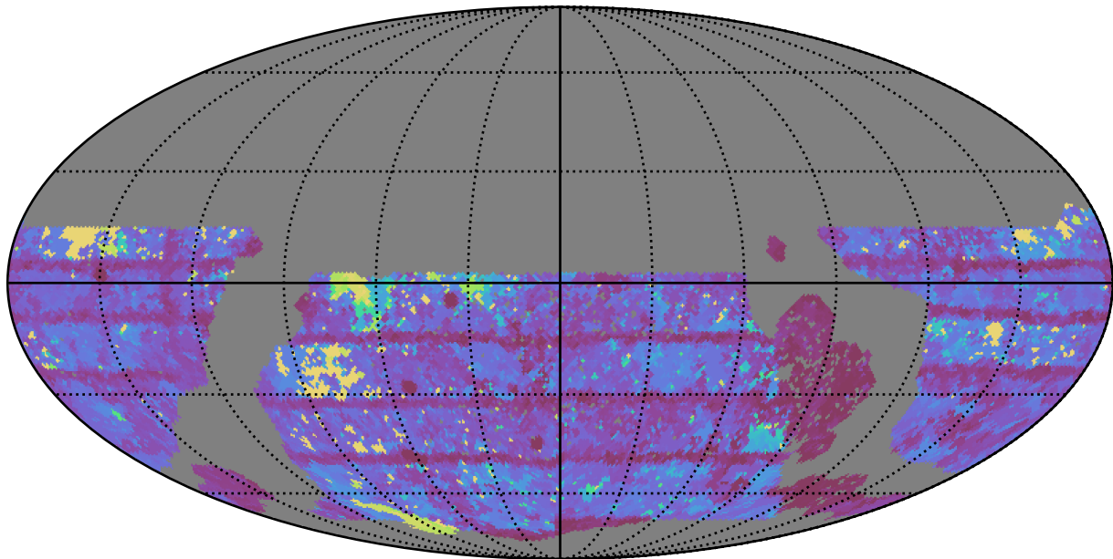
ddf_loaded_fl8_v3.4_10yrs WFD i band: Max Inter-Night Gap
