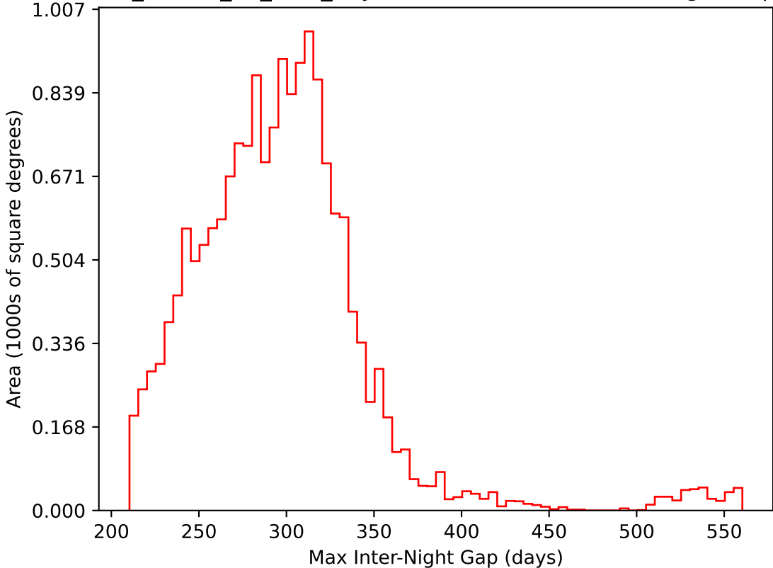
ddf_loaded_fl8_v3.4_10yrs WFD i band: Max Inter-Night Gap
