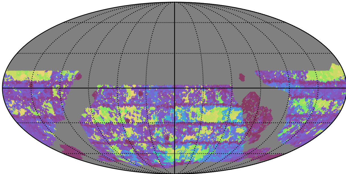
ddf_loaded_fl8_v3.4_10yrs WFD g band: Max Inter-Night Gap
