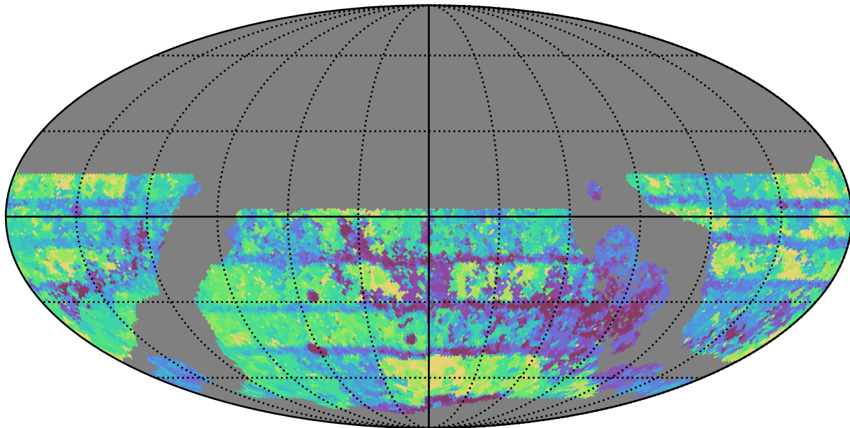
ddf_loaded_fl8_v3.4_10yrs WFD all bands: Max Inter-Night Gap
