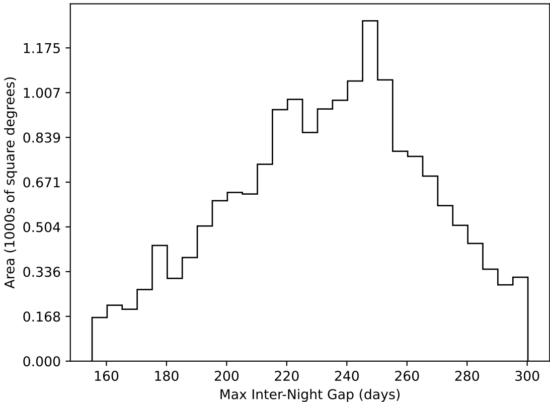
ddf_loaded_fl8_v3.4_10yrs WFD all bands: Max Inter-Night Gap
