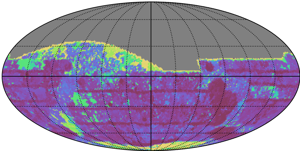
ddf_loaded_fl8_v3.4_10yrs All sky z band: Max Inter-Night Gap
