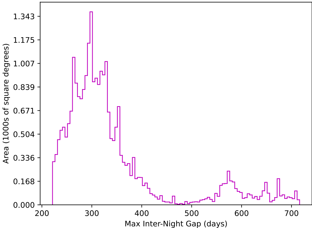
ddf_loaded_fl8_v3.4_10yrs All sky z band: Max Inter-Night Gap
