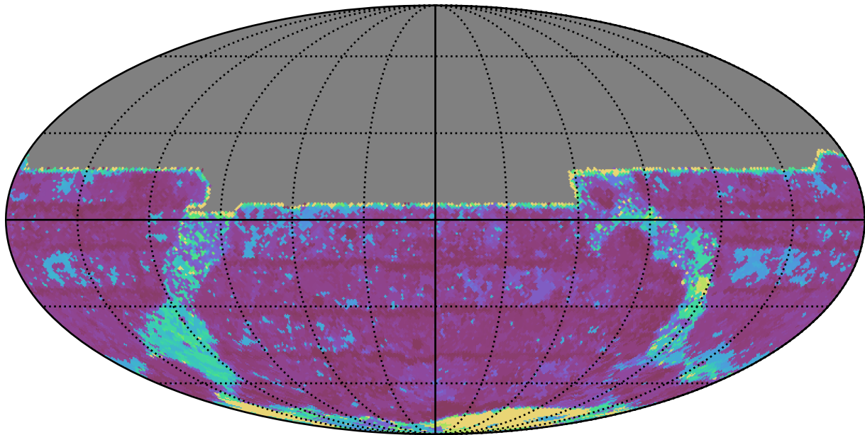
ddf_loaded_fl8_v3.4_10yrs All sky y band: Max Inter-Night Gap
