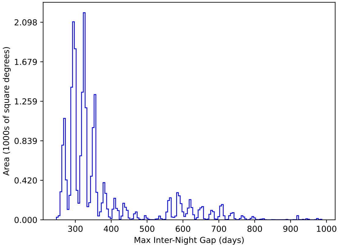
ddf_loaded_fl8_v3.4_10yrs All sky y band: Max Inter-Night Gap
