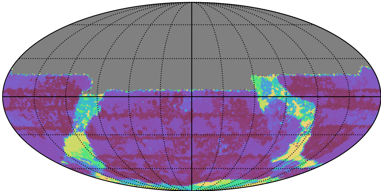
ddf_loaded_fl8_v3.4_10yrs All sky u band: Max Inter-Night Gap
