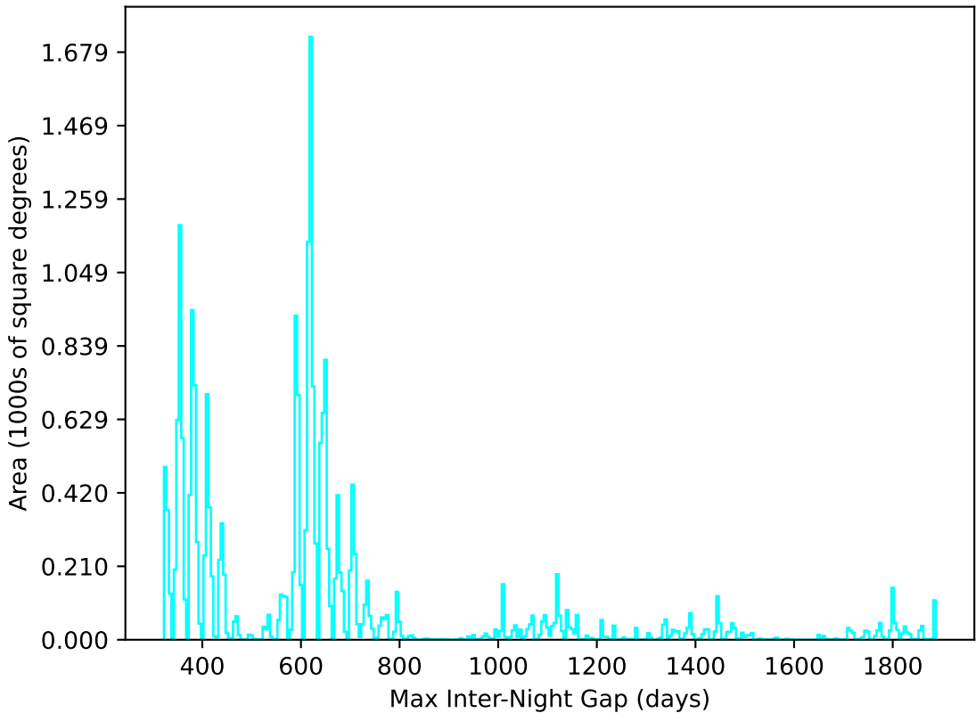
ddf_loaded_fl8_v3.4_10yrs All sky u band: Max Inter-Night Gap
