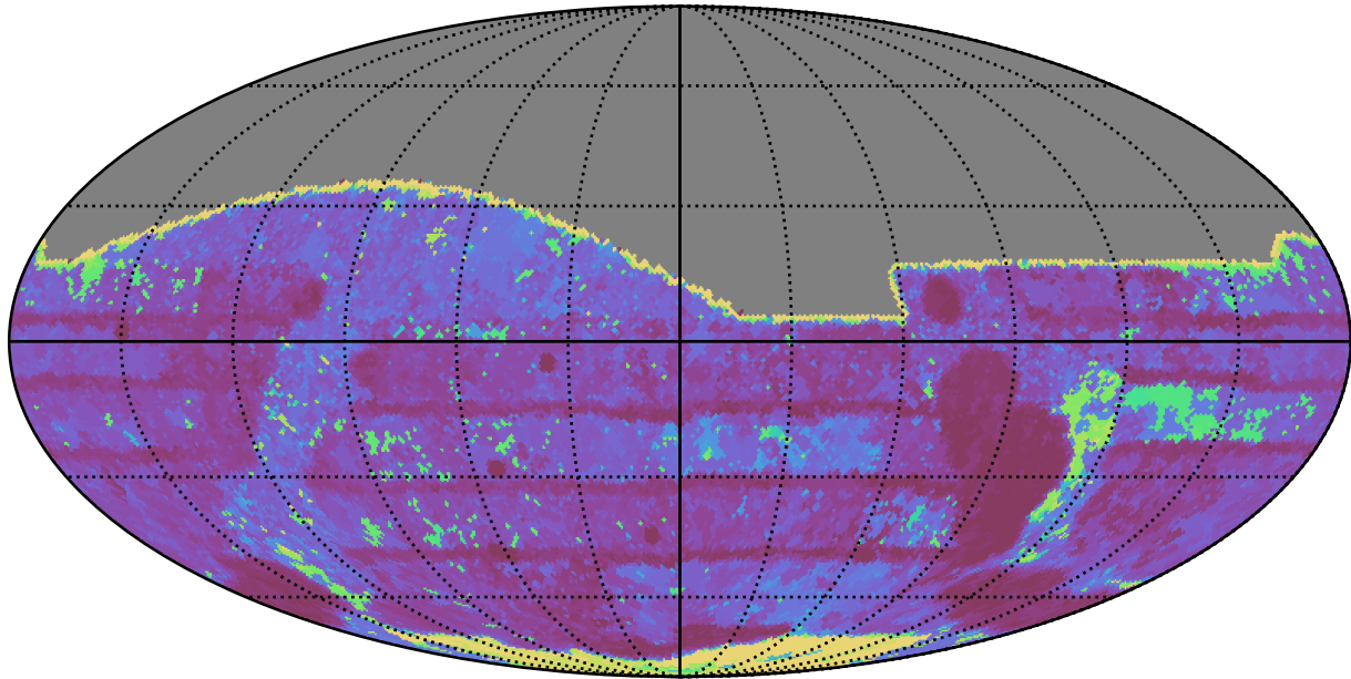
ddf_loaded_fl8_v3.4_10yrs All sky r band: Max Inter-Night Gap
