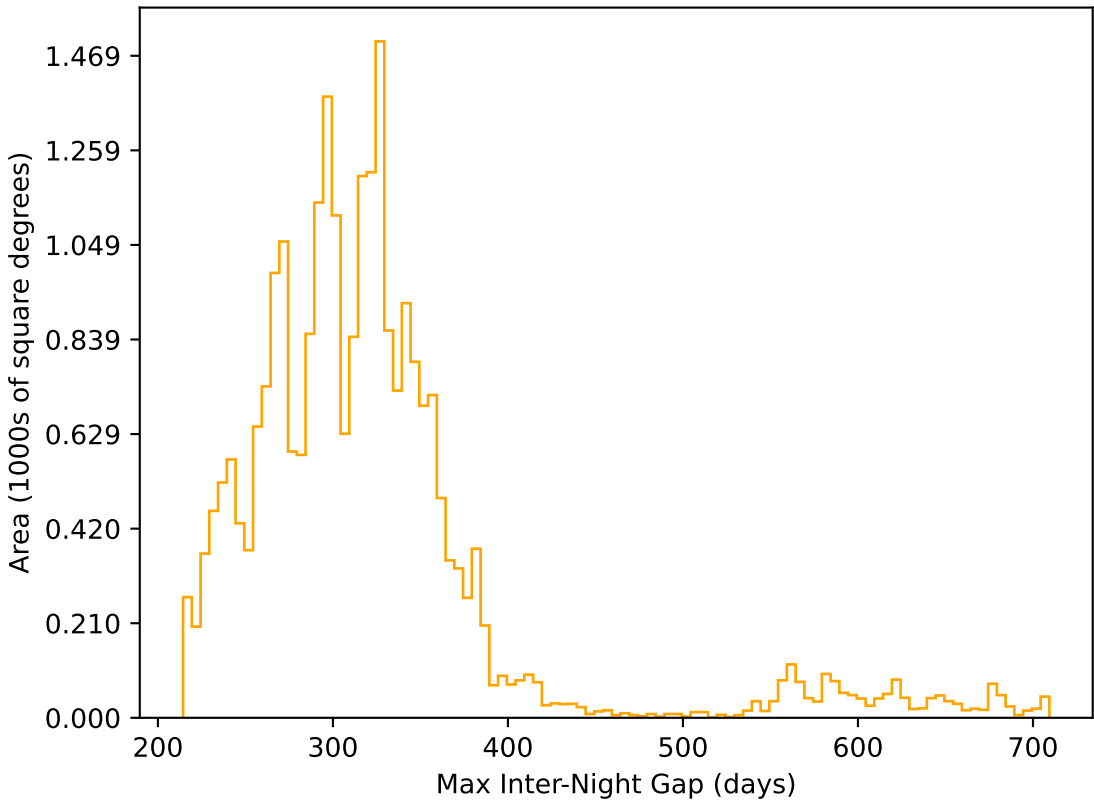
ddf_loaded_fl8_v3.4_10yrs All sky r band: Max Inter-Night Gap
