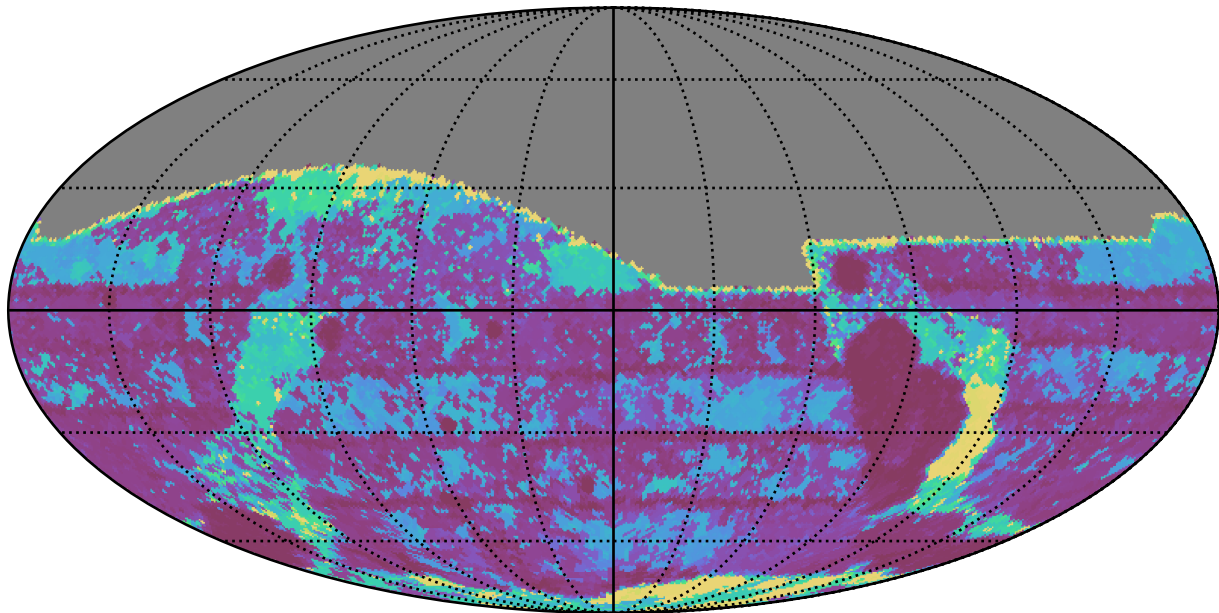
ddf_loaded_fl8_v3.4_10yrs All sky g band: Max Inter-Night Gap
