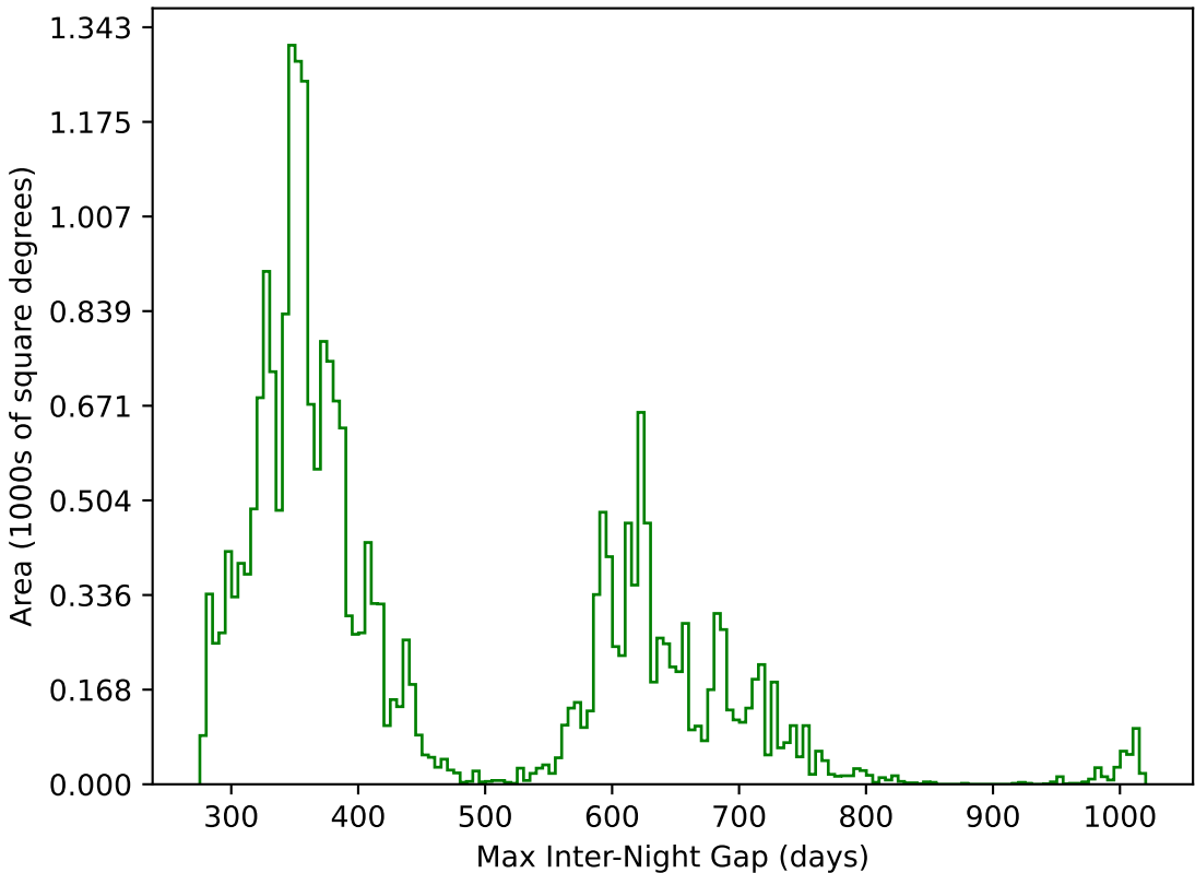
ddf_loaded_fl8_v3.4_10yrs All sky g band: Max Inter-Night Gap
