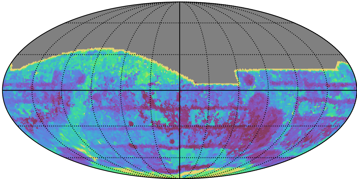
ddf_loaded_fl8_v3.4_10yrs All sky all bands: Max Inter-Night Gap
