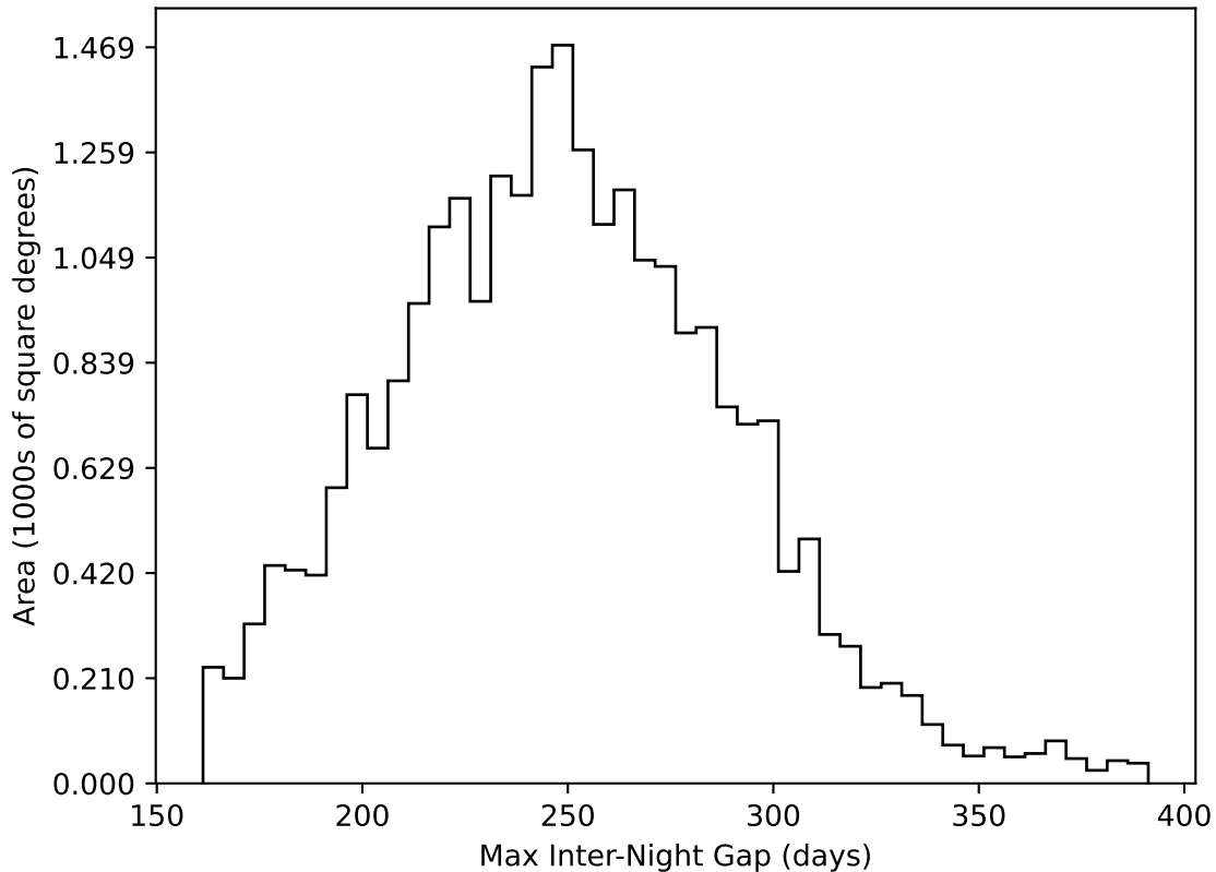
ddf_loaded_fl8_v3.4_10yrs All sky all bands: Max Inter-Night Gap
