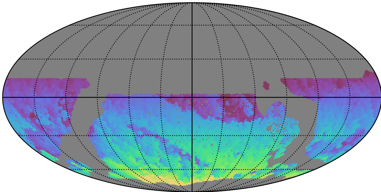
ddf_loaded_fl8_v3.4_10yrs WFD z band: Max HA
