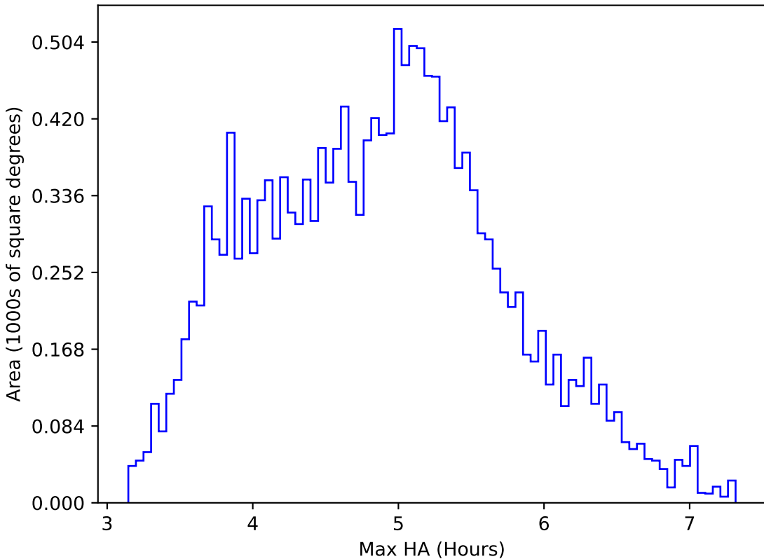
ddf_loaded_fl8_v3.4_10yrs WFD z band: Max HA
