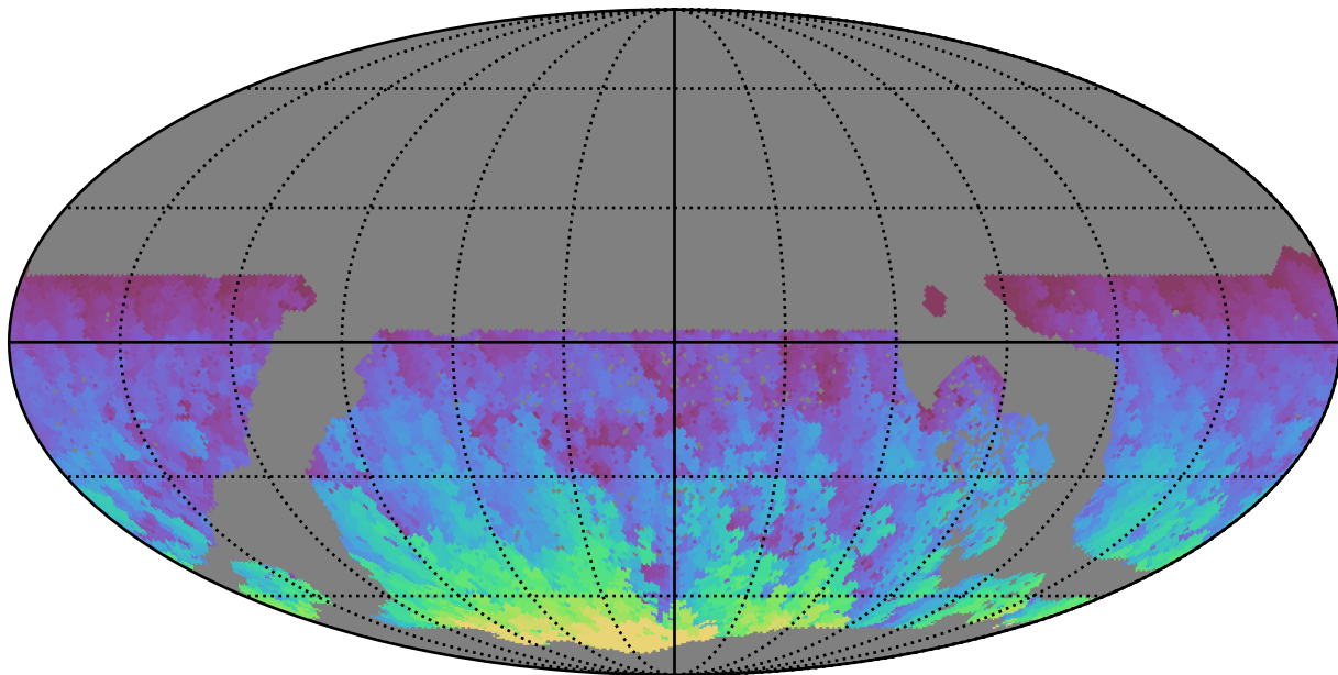
ddf_loaded_fl8_v3.4_10yrs WFD y band: Max HA
