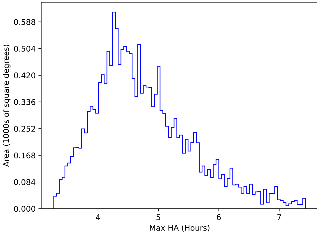
ddf_loaded_fl8_v3.4_10yrs WFD y band: Max HA
