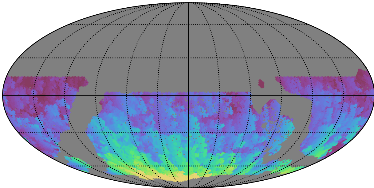
ddf_loaded_fl8_v3.4_10yrs WFD r band: Max HA
