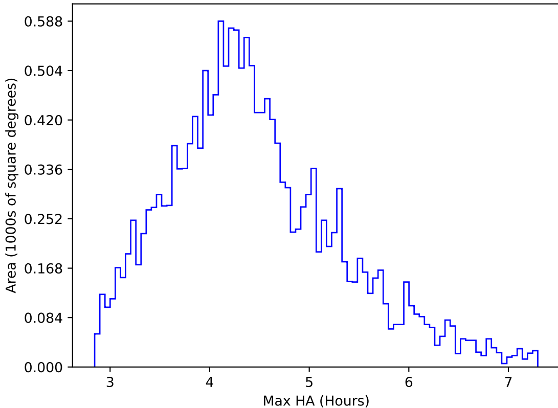
ddf_loaded_fl8_v3.4_10yrs WFD r band: Max HA
