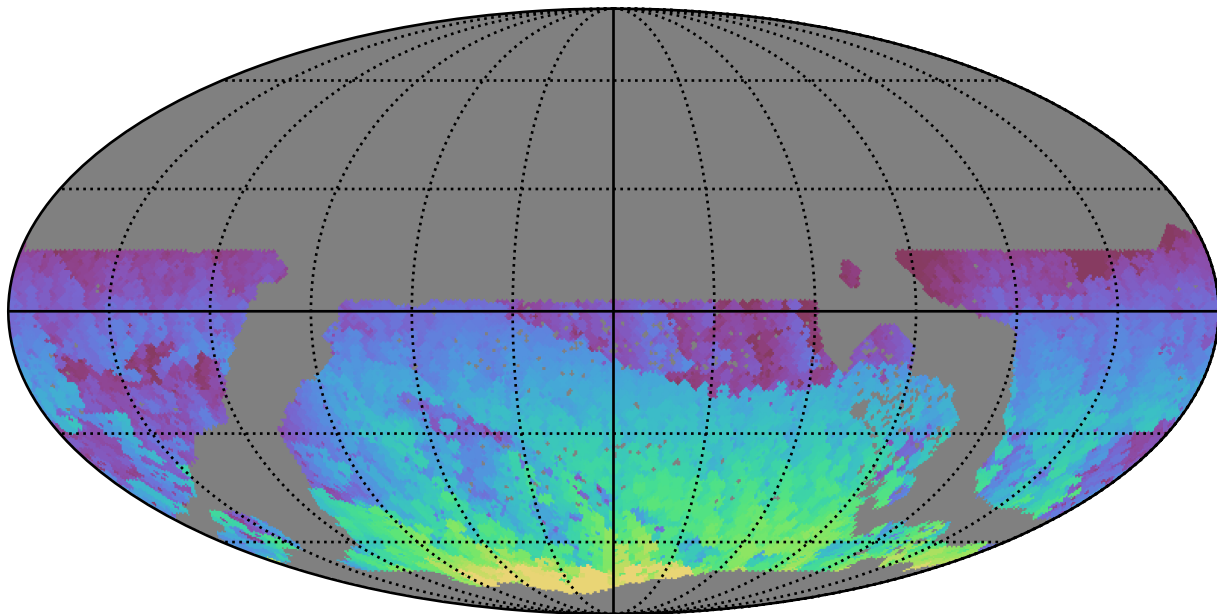
ddf_loaded_fl8_v3.4_10yrs WFD i band: Max HA
