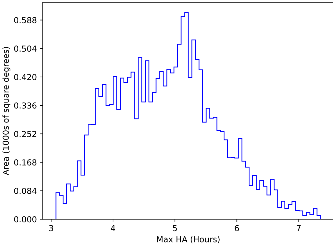
ddf_loaded_fl8_v3.4_10yrs WFD i band: Max HA
