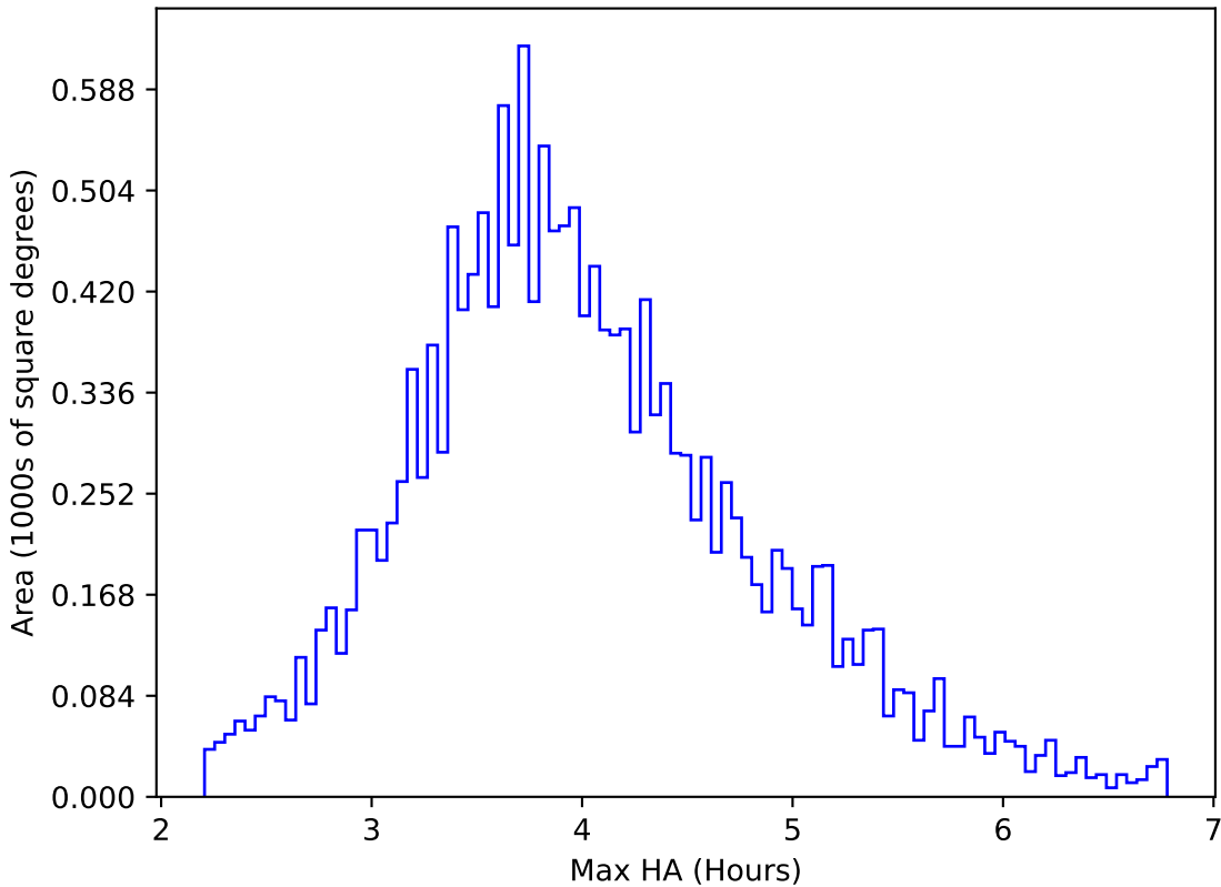
ddf_loaded_fl8_v3.4_10yrs WFD g band: Max HA
