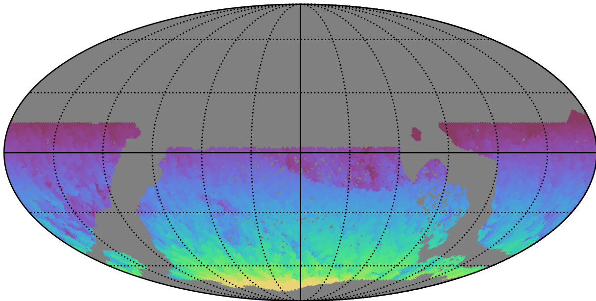
ddf_loaded_fl8_v3.4_10yrs WFD all bands: Max HA
